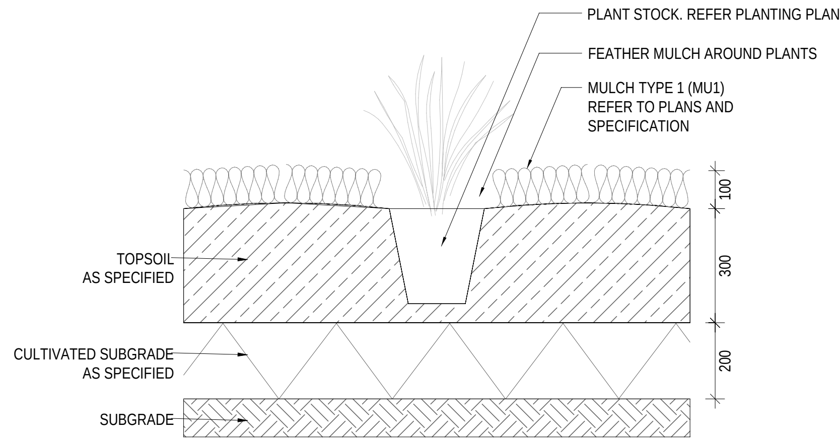
1 GARDEN BED TYPE 1 - PLANTING ON NATURAL GROUND SCALE - 1 : 10
