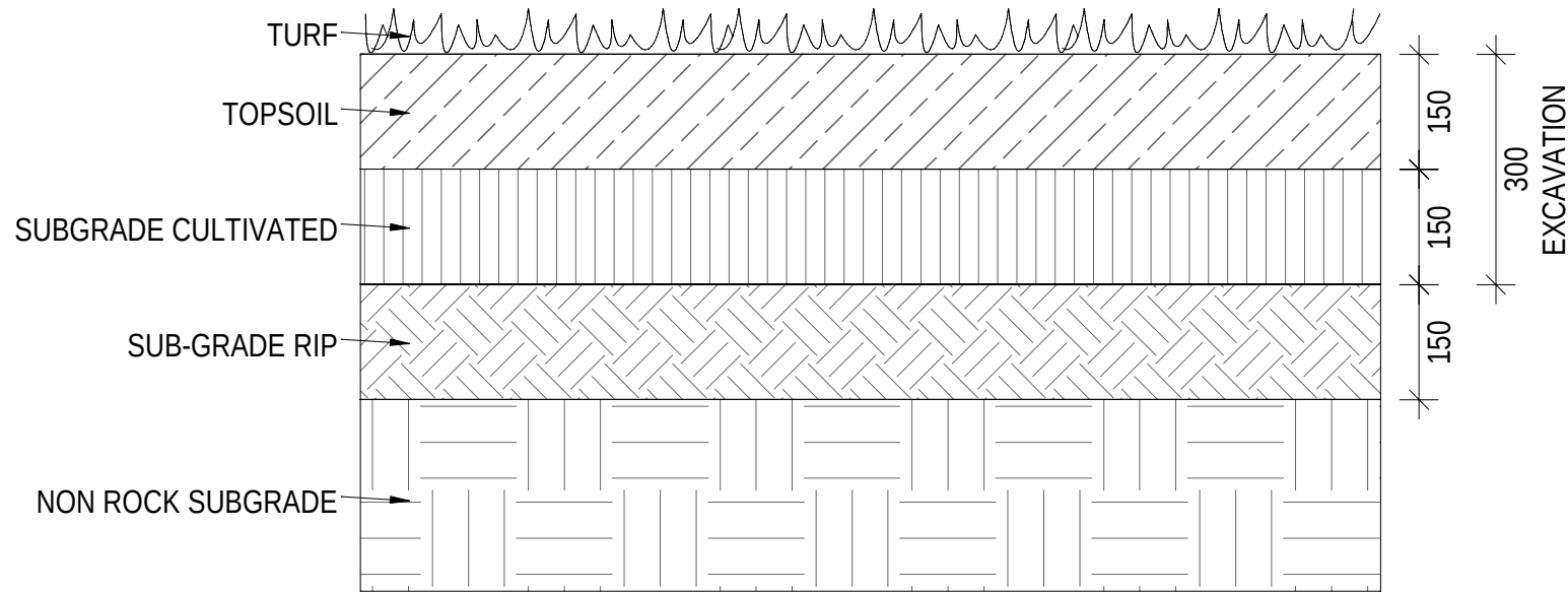
2 TURF TYPE 1 - TURF ON NATURAL GROUND SCALE - 1 : 10
