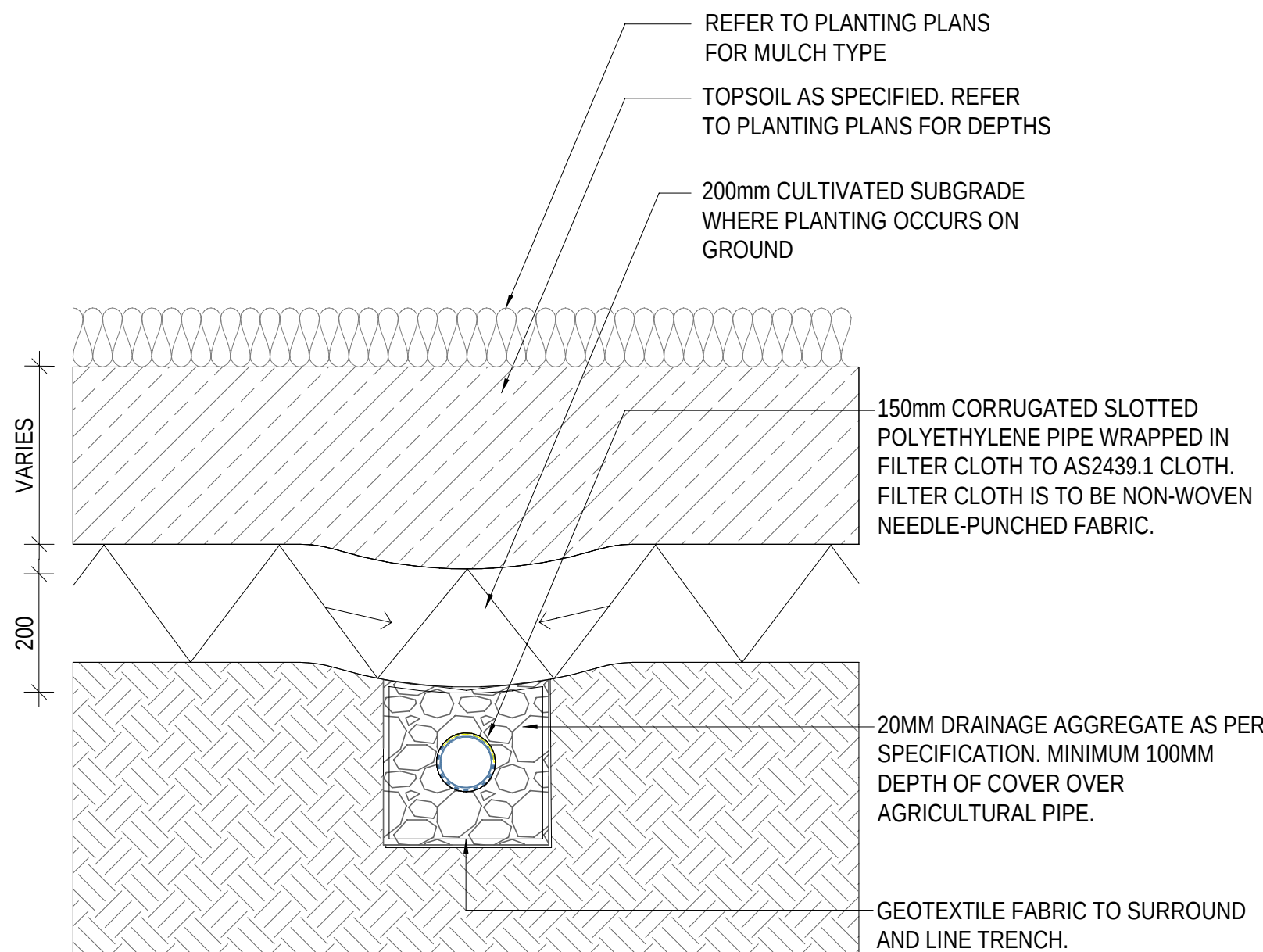
3 SUB SOIL DRAINAGE - PLANTING ON NATURAL GROUND SCALE - 1 : 10
